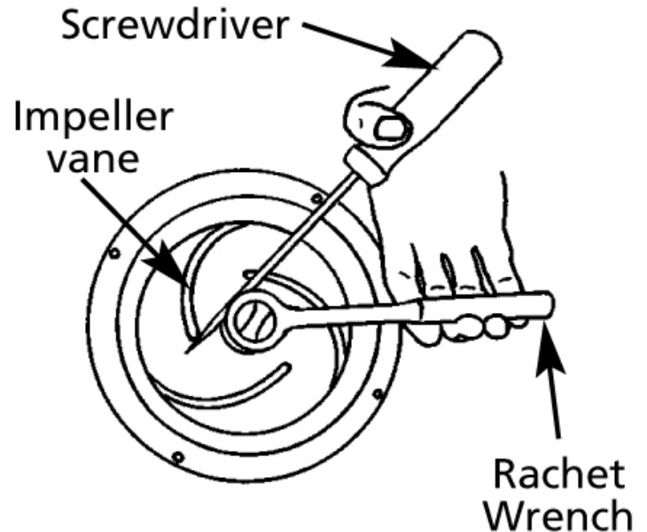
Figure 1 - Impeller Removal
